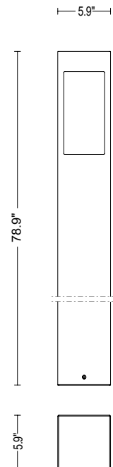
Fixture Dimensions
