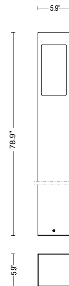
Fixture Dimensions
