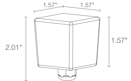
Fixture Dimensions
