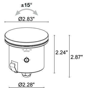
Fixture Dimensions
