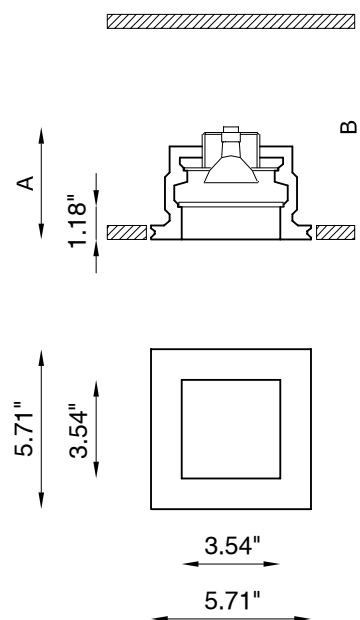
Fixture Dimensions
