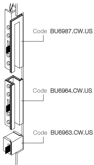
1 electrified body 1 modular body 1 closure headpart
