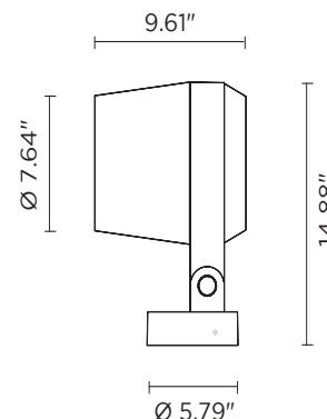
Fixture Dimensions
