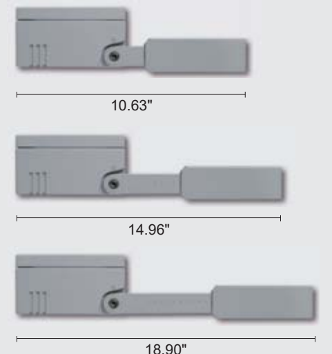
AC003: Wall extensible bracket Die-cast aluminum (option to be ordered separately)
