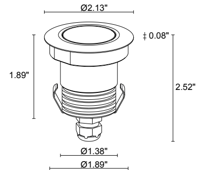
Fixture Dimensions
