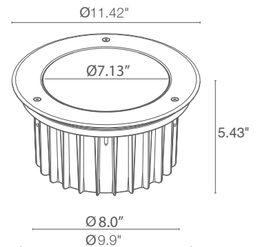
Fixture Dimensions
