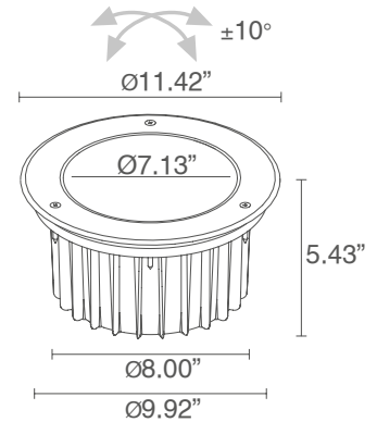
Fixture Dimensions
