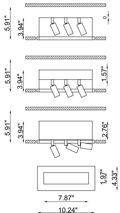
Fixture Dimensions
