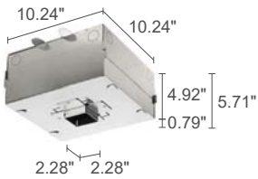
WC3101 Outer casing for solid walls (Turis 1.0 / 1.2)
