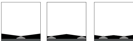
170° SINGLE INSTALLATION, IN THE MIDDLE: SUGGESTED FOR SMALL / MEDIUM SIZE WINDOWS 170° DOUBLE INSTALLATION, ON BOTH SIDES: SUGGESTED IN CASE OF HIGH LIGHTING PERFORMANCE NEEDED 170° DOUBLE INSTALLATION, IN THE MIDDLE: SUGGESTED FOR BIG SIZE WINDOWS
