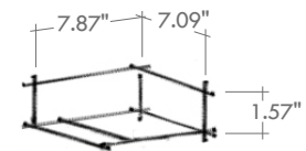
Fixture Dimensions
