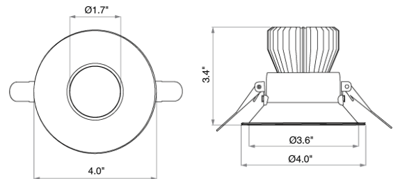
Fixture Dimensions
