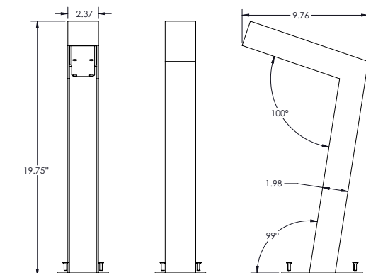
Fixture Dimensions
