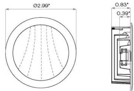
Fixture Dimensions
