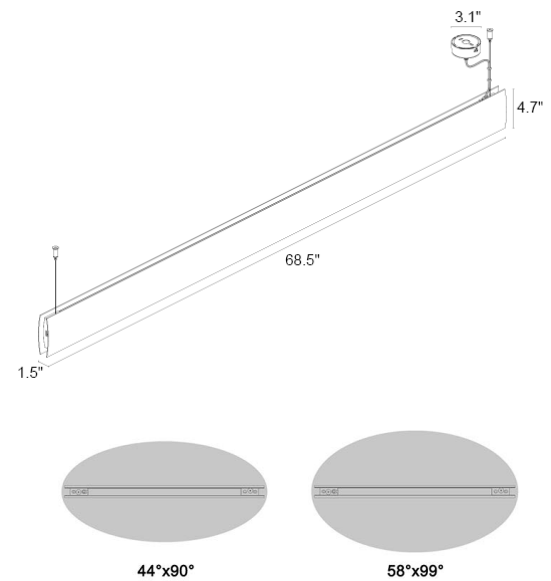
Fixture Dimensions
