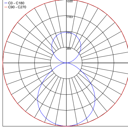
PHOTOMETRIC FILENAME : BERICA_S_2.2_L_3000K_39W.IES
