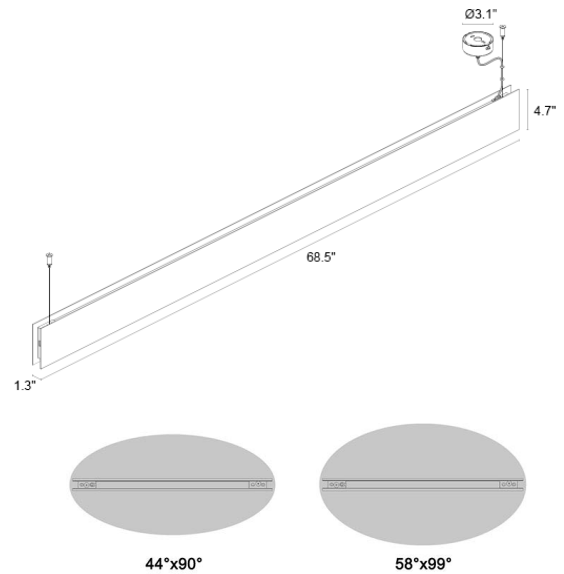
Fixture Dimensions
