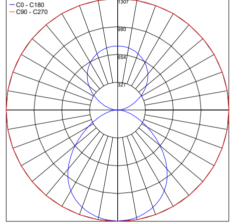
PHOTOMETRIC FILENAME : BERICA_S_2.2_K_3000K_39W.IES
