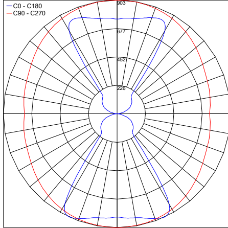
PHOTOMETRIC FILENAME : BERICA_S_2.2_D_3000K_39W.IES
