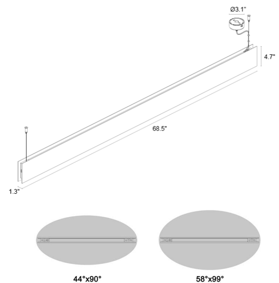
Fixture Dimensions
