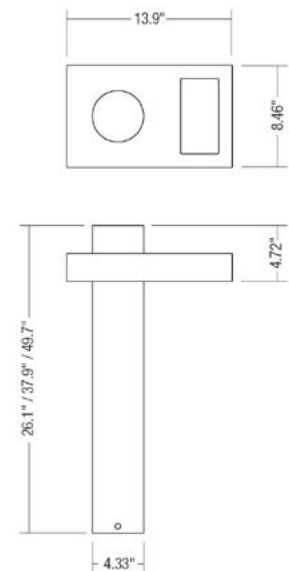
Fixture Dimensions
