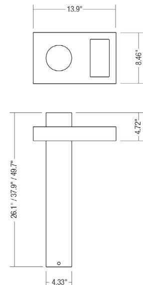
Fixture Dimensions
