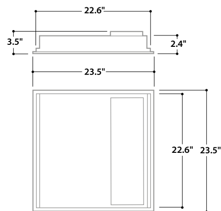
Fixture Dimensions
