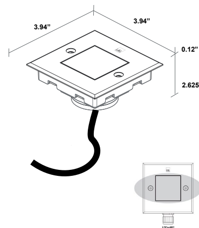
Fixture Dimensions
