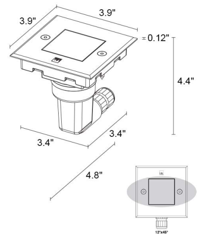
Fixture Dimensions
