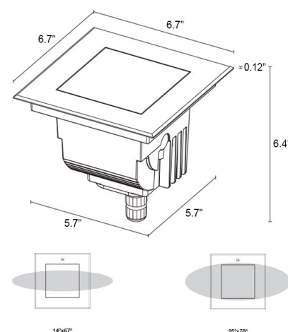
Fixture Dimensions
