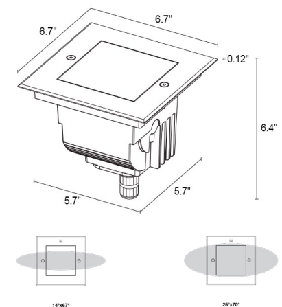
Fixture Dimensions
