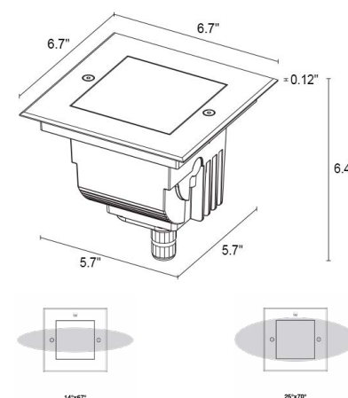
Fixture Dimensions
