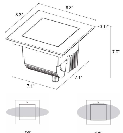
Fixture Dimensions
