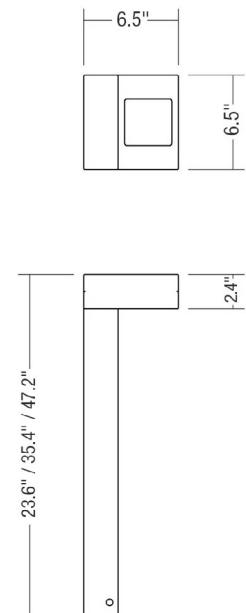
Fixture Dimensions
