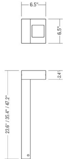
Fixture Dimensions
