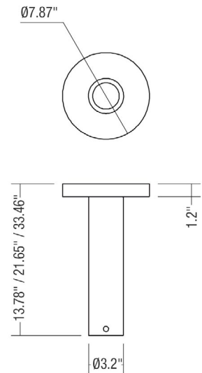
Fixture Dimensions
