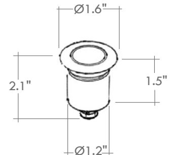
Fixture Dimensions
