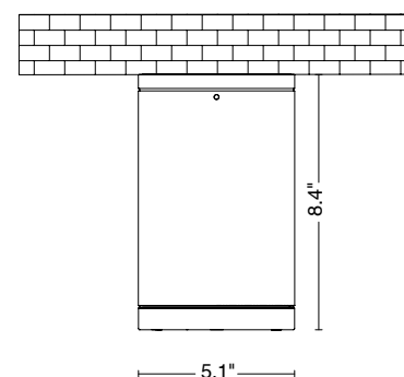
Fixture Dimensions
