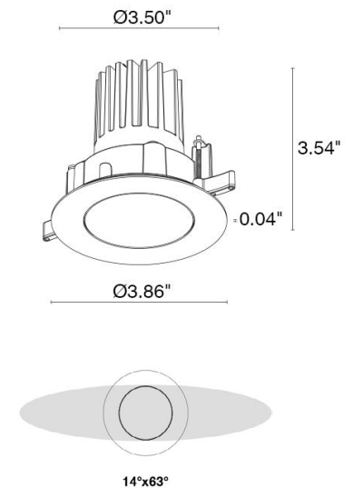
Fixture Dimensions
