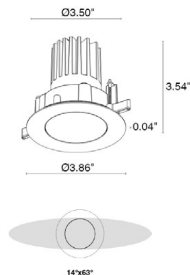
Fixture Dimensions
