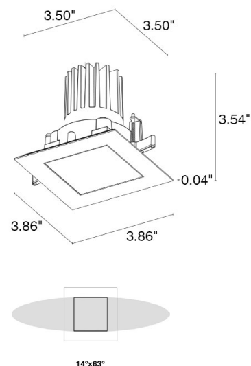
Fixture Dimensions
