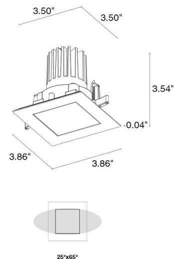
Fixture Dimensions
