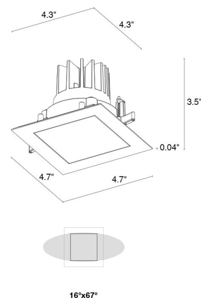
Fixture Dimensions
