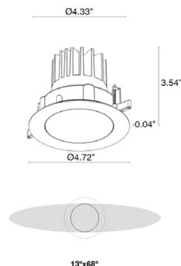
Fixture Dimensions
