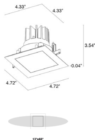
Fixture Dimensions
