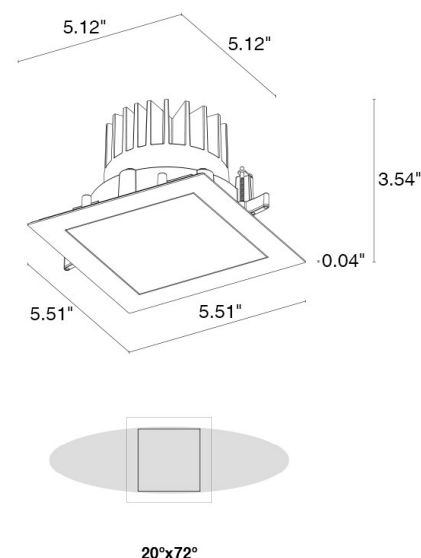
Fixture Dimensions
