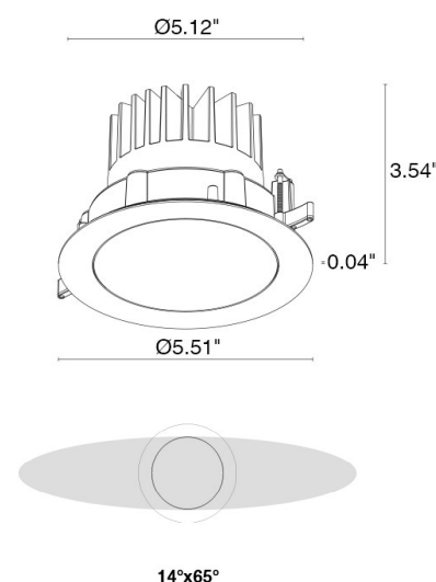
Fixture Dimensions
