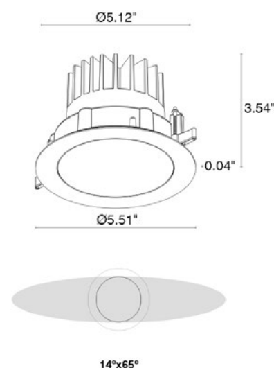
Fixture Dimensions
