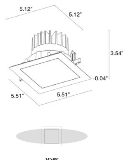
Fixture Dimensions
