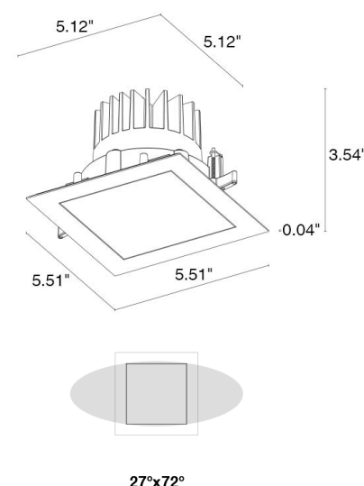
Fixture Dimensions
