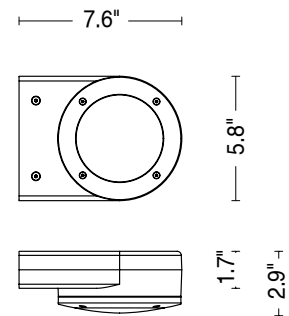
Fixture Dimensions
