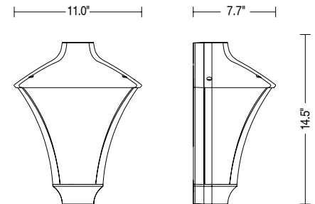
Fixture Dimensions
