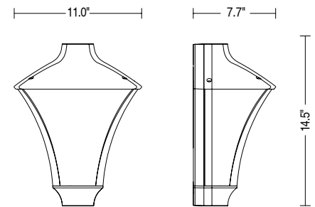
Fixture Dimensions
